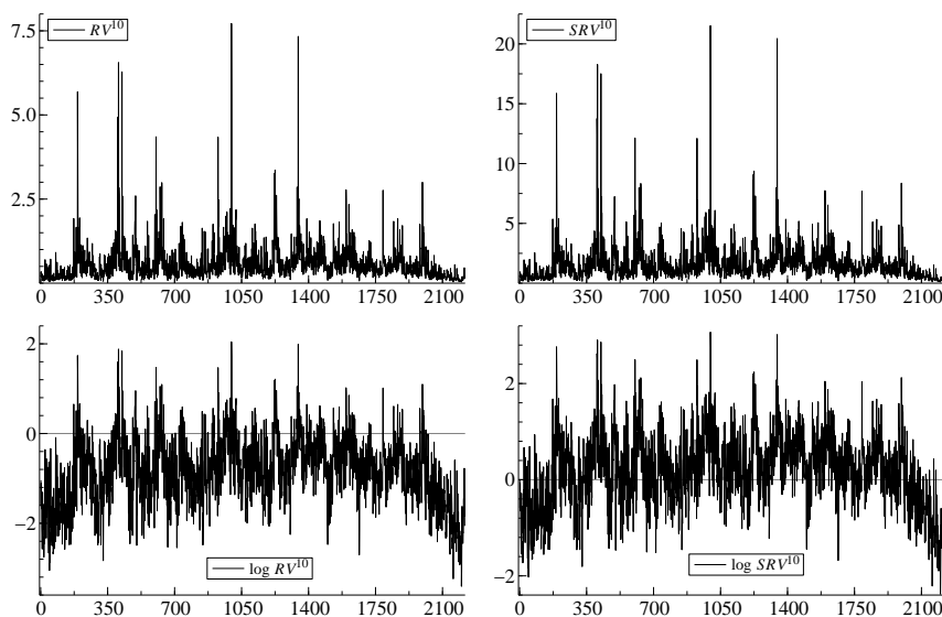
Fig. 3. Realized volatility calculated from 10-minute intraday returns ( RV^{10} , top left), scaled one ( SRV^{10} , top right), and their logarithms ( \log RV^{10} , bottom left; \log SRV^{10} , bottom right) during the period from April 1, 1996 to March 31, 2005 (2216 trading days).
