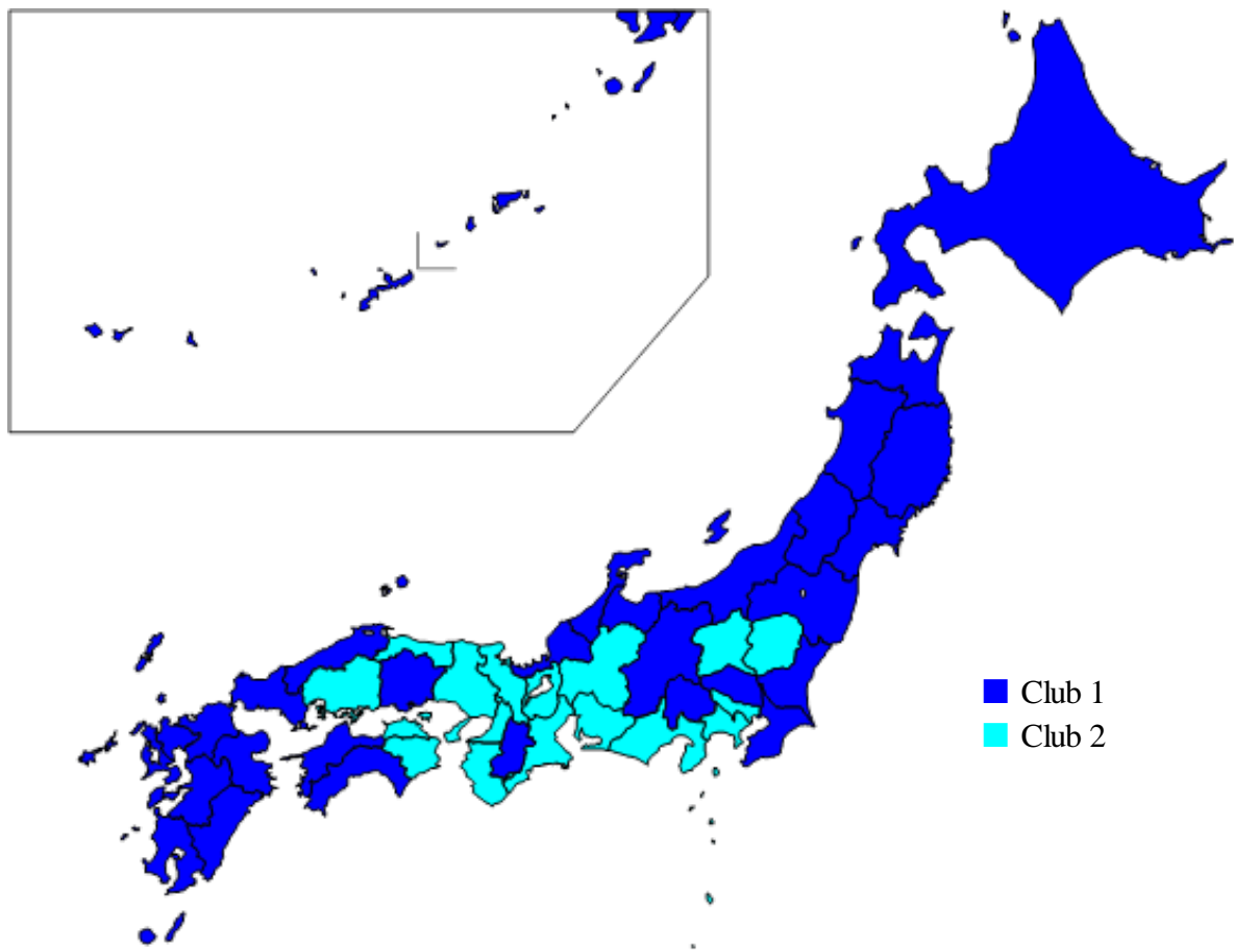
Figure5: Club convergence test for the subperiods
