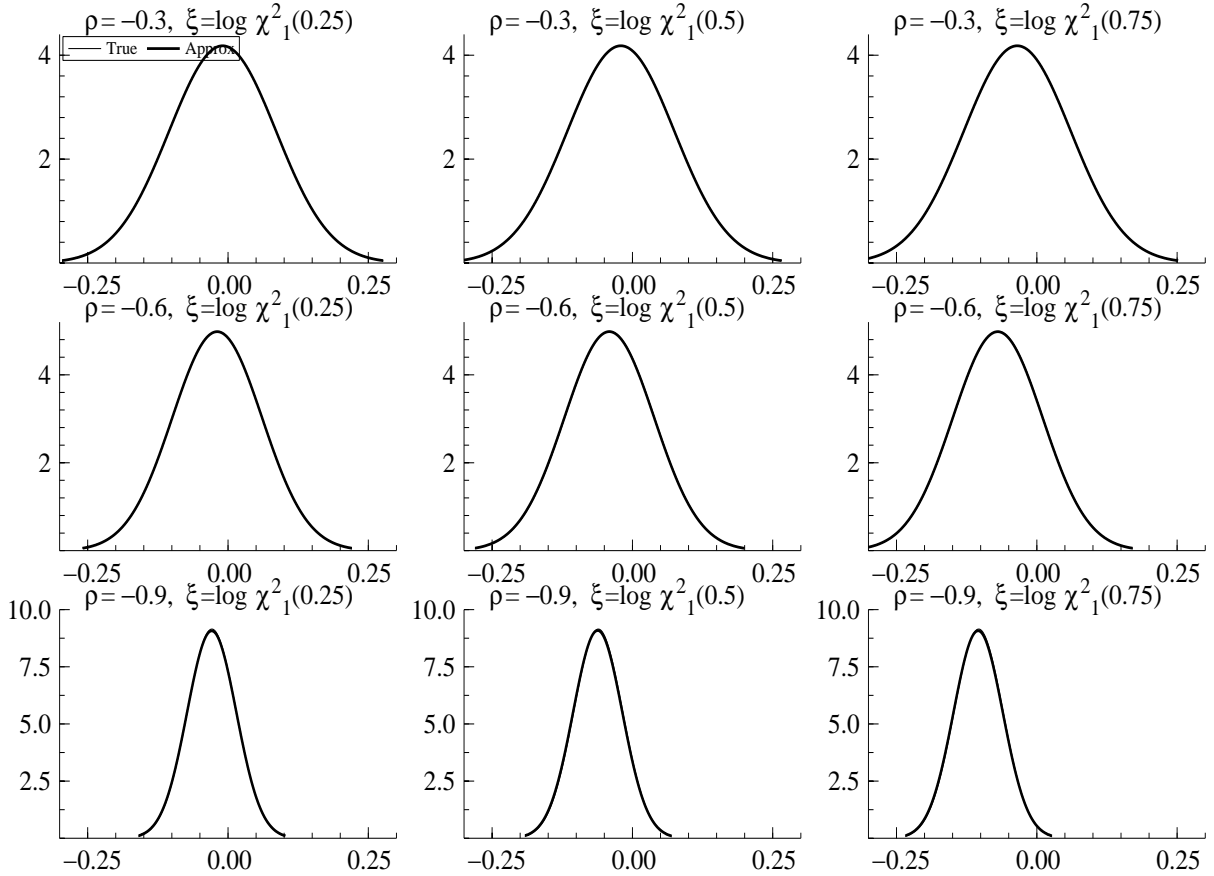
Figure 2: The conditional density of \eta_t given d_t = 1 and v_t = \log \chi_1^2(0.25), \log \chi_1^2(0.5), \log \chi_1^2(0.75) (left, middle, right) for \rho = -0.3, -0.6, -0.9 (top, middle, bottom).
