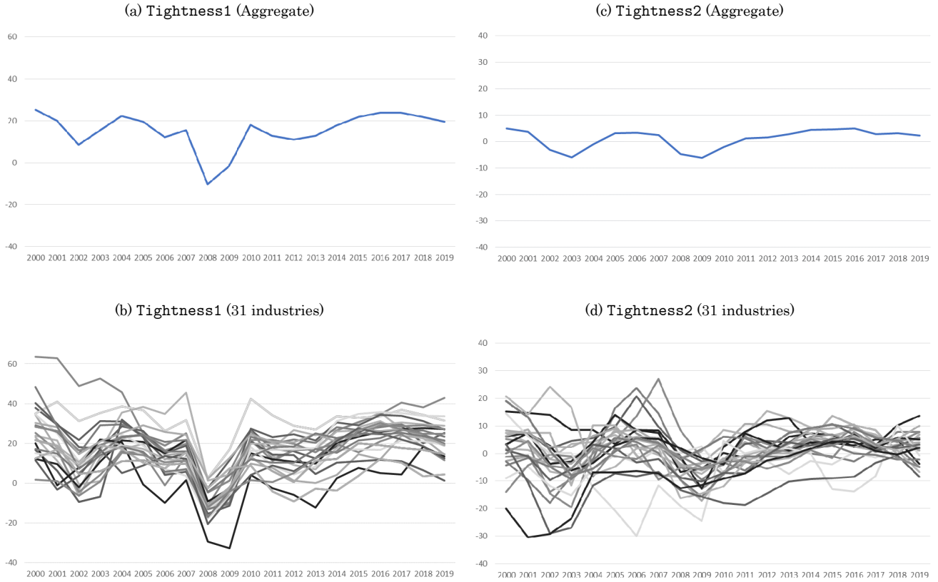
Figure 3: Time series plot of the credit market tightness
